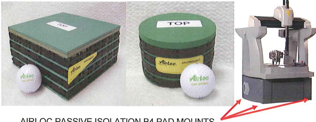
AIRLOC PASSIVE ISOLATION B4 PAD MOUNTS
