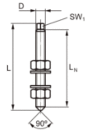
Dimensioned sketch
